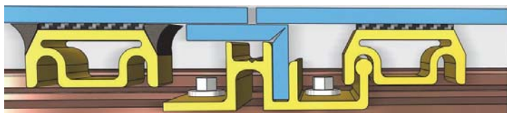
Arrowhead® Flush Panel System Non-Progressive
