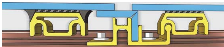
Arrowhead® Flush Panel System Non-Progressive
