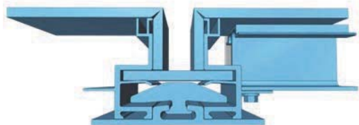
Arrowhead® Rainscreen 1" Insulated
