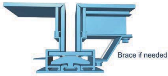
Arrowhead® Rainscreen Custom Depth
